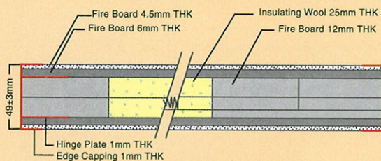
SECTION A-A CROSS SECTION OF DOOR LEAF
