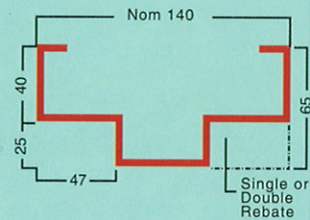
TYPICAL METAL DOOR JAMB SECTION
