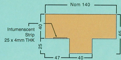
TYPICAL TIMBER DOOR JAMB SECTION
