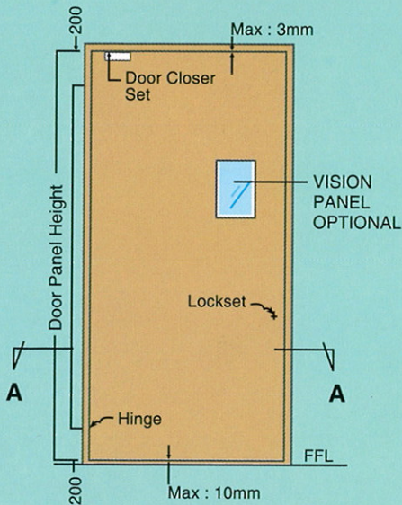
DOOR LEAF MAXIMUM SIZE : 1220 x 2440mm
