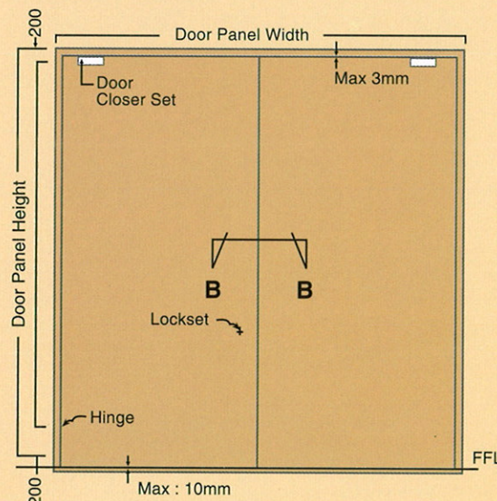
DOOR LEAF MAXIMUM SIZE : 2440 x 2440mm
