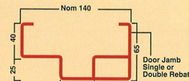
TYPICAL METAL DOOR JAMB SECTION
