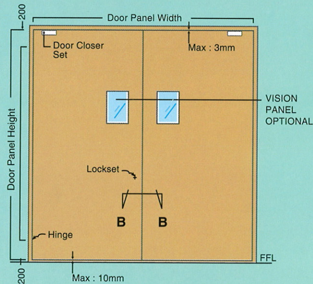
DOOR LEAF MAXIMUM SIZE : 2440 x 2440mm
