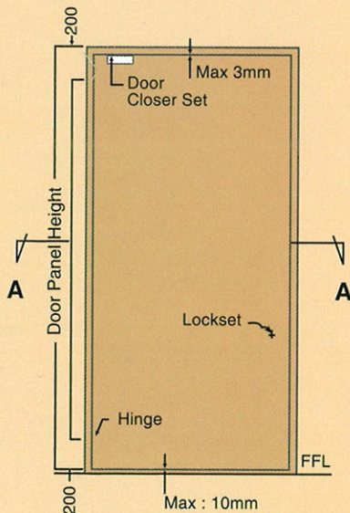
DOOR LEAF MAXIMUM SIZE : 1220 x 2440mm
